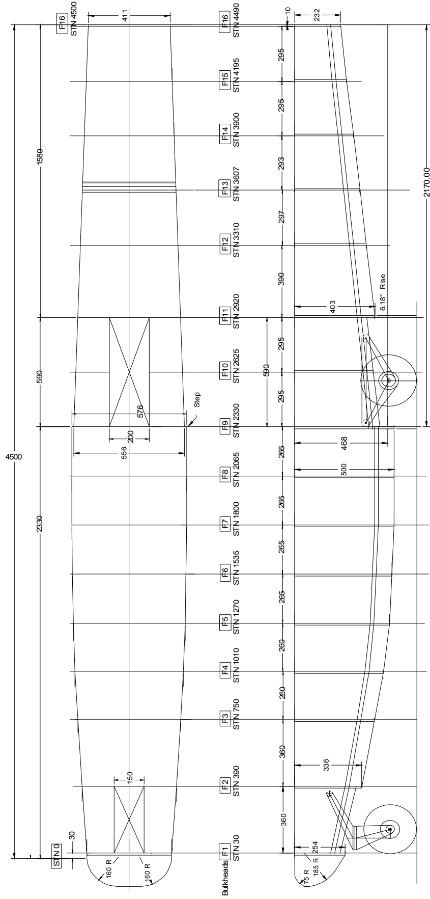
1200 Size Amphibious Floats
